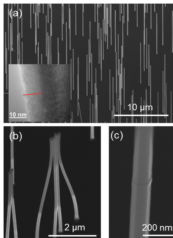
FIG. 1. p - i - n Si NWs grown from 100 nm Au nanoparticles: (a) and (b) 30 °-tilted view of the NW arrays. Contrast in (b) reveals the doping profile along the NW axis (due to charging effects, the initially isolated Si NWs collapsed under the e-beam upon SEM analysis); (c) small bulge on the NW trunk which forms during growth interruption. Inset in (a) shows a high-resolution TEM image of a passivated wire with a \sim 12 \text{ nm} \text{SiO}_2 sheath, indicated by the red marker.
