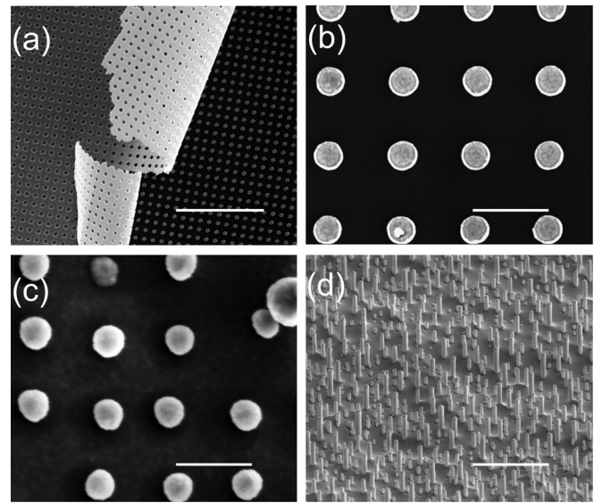
FIG. 7. Nanoimprint lithography for dense NW array growth: (a) MR-I 7020E resist lift-off, leaving behind a square array of 30 nm thick gold particles; (b) close-up of NIL-arranged gold seed particles with P = 500 \text{ nm} and diameter of \sim 150 \text{ nm} ; (c) top-view of NW array, with some NWs missing or merged during the growth, resulting in a lower final NW density than the nanoimprint maximum; (d) 52°-tilted view of NW array after IZO top contact deposition. Scale bars are 5 \mu\text{m} for (a) and (d) and 500 nm for (b) and (c).
