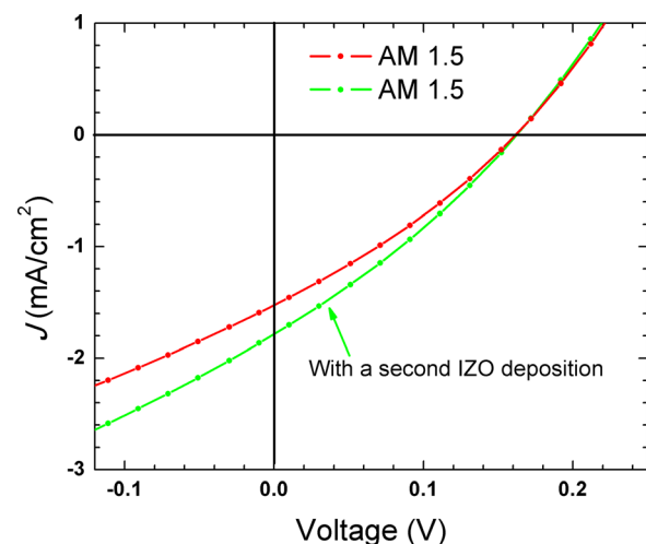
FIG. 8. Photovoltaic performance of sample B under AM 1.5G illumination. The green dashed line shows a 15% improvement on J_{\text{SC}} after a second deposition of IZO top contact with the sample tilted at a small angle with respect to the IZO source.
