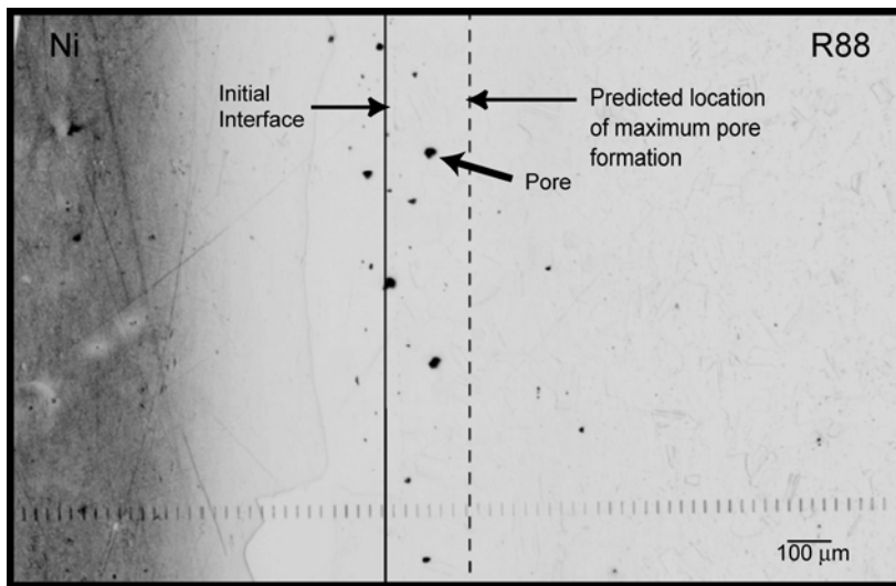
Ni/René-88 at 1150 °C for 1000 h
