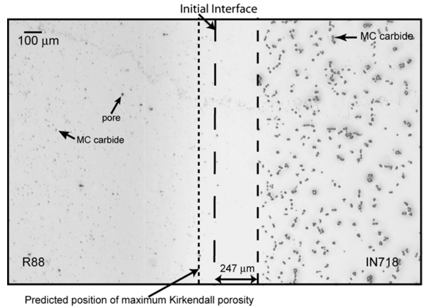
René-88/IN-718 at 1150 °C for 1000 h
