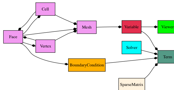
Fig. 7.1: Primary object relationships in FiPy .
